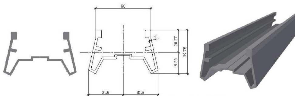
Figure 9 – Éclisses
