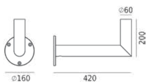
Art. 154 Fixation murale ø60 Asker Head Borg Hammerfest Mora Visby
